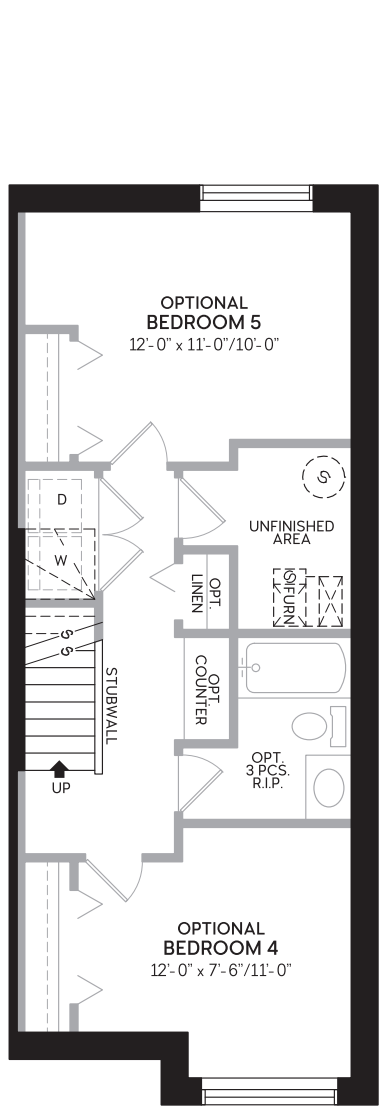
BASEMENT OPTIONAL DEVELOPMENT 460 SQ.FT.
