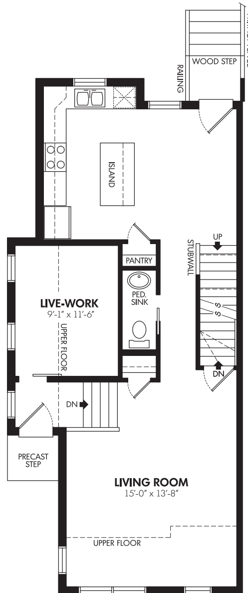
MAIN FLOOR 820 SQ.FT.
