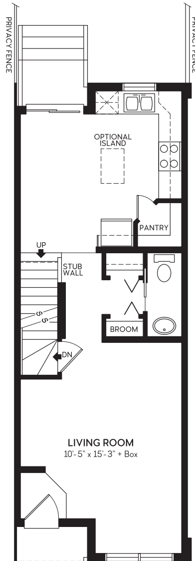
MAIN FLOOR 589 SQ.FT.
