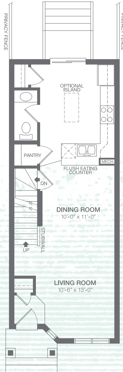
MAIN FLOOR 579 sq.ft.
