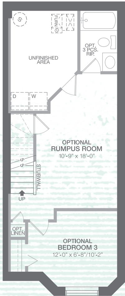
BASEMENT OPTIONAL DEVELOPMENT 377 sq.ft.
