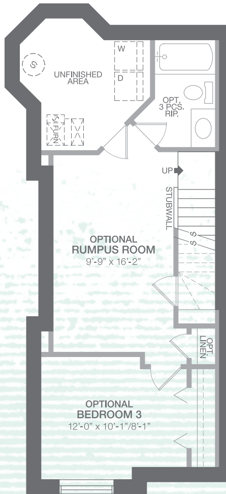
BASEMENT OPTIONAL DEVELOPMENT 377 sq.ft.
