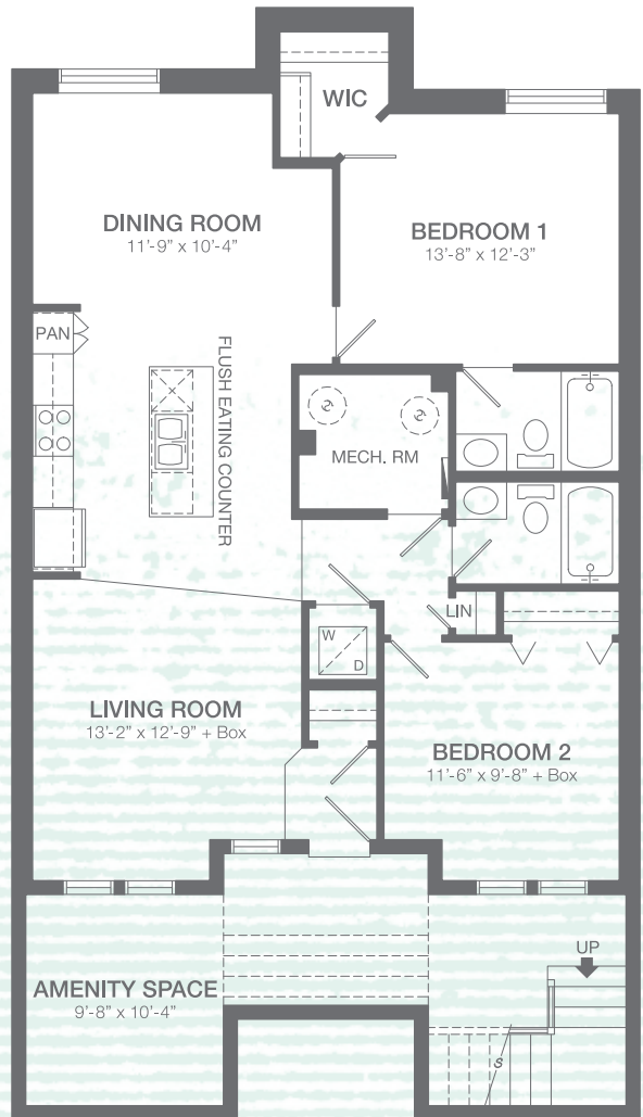
STANDARD OPTION 1059 sq.ft.
